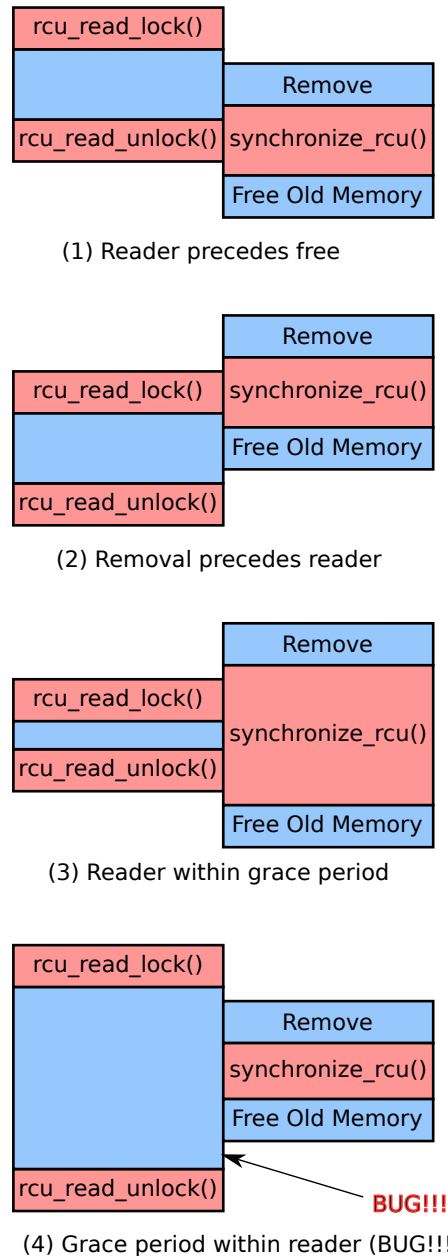
Figure 9.15: Summary of RCU Grace-Period Ordering Guarantees
