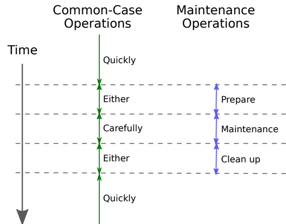
Figure 9.25: Phased State Change for Maintenance Operation
