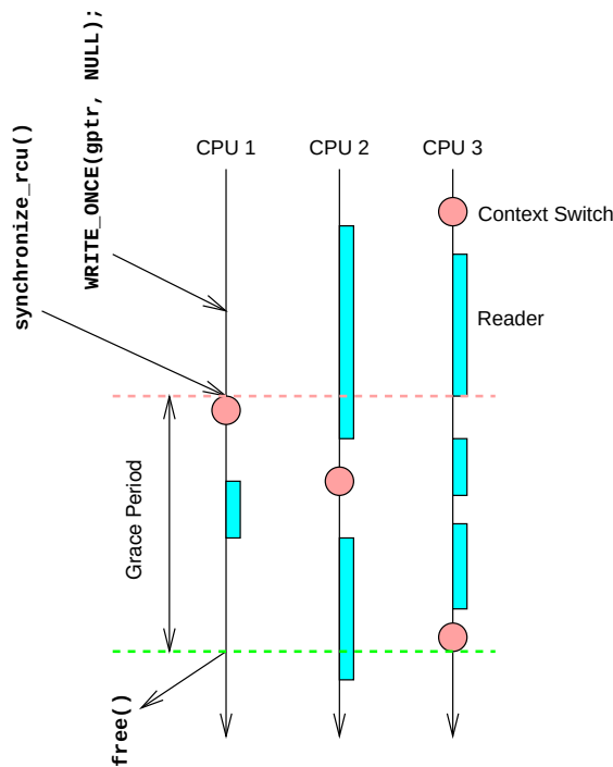
Figure 9.9: QSBR: Waiting for Pre-Existing Readers
