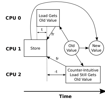
Figure E.11: Is Load-to-Store Counter-Temporal on x86?
