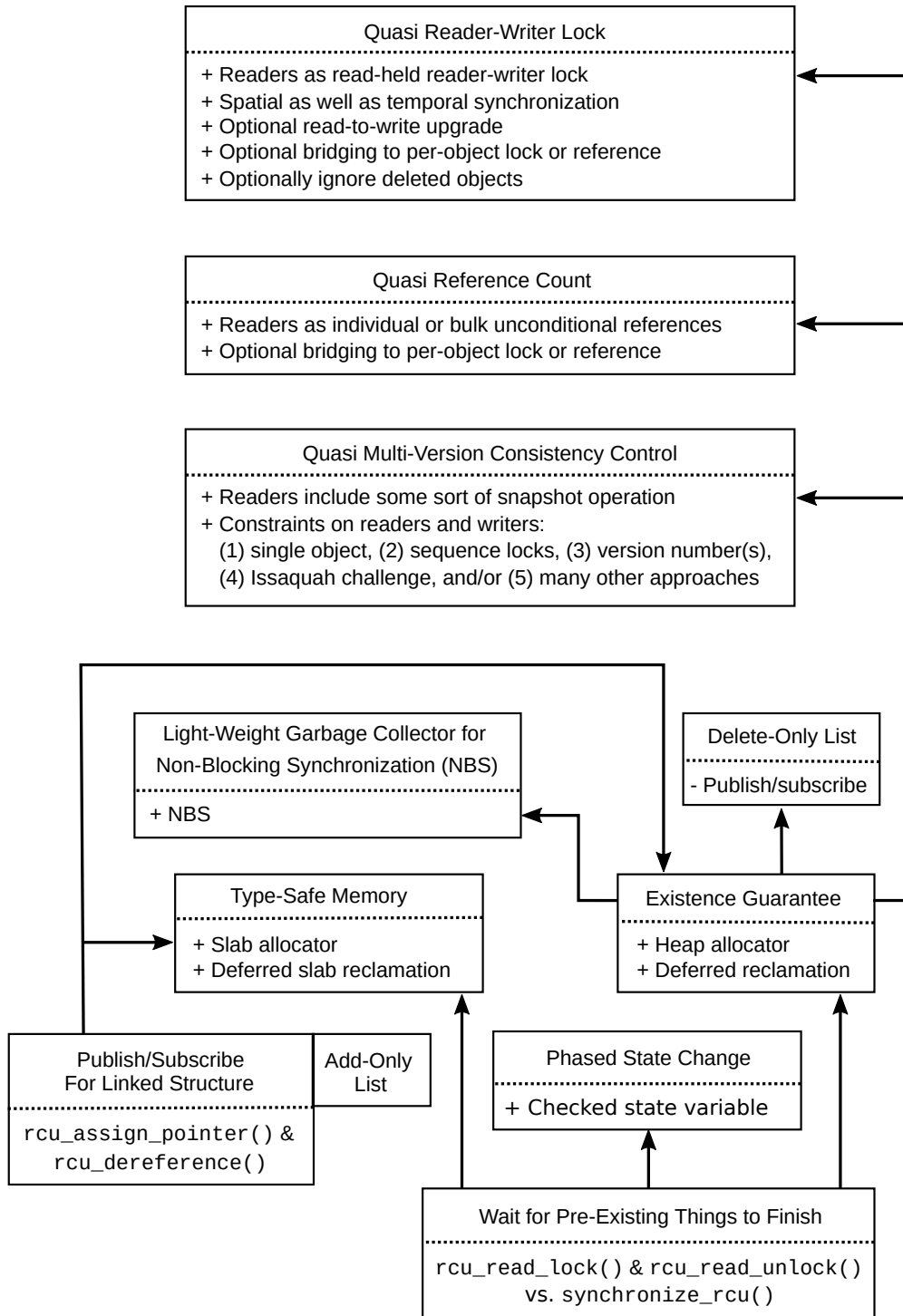
Figure 9.24: Relationships Between RCU Use Cases
