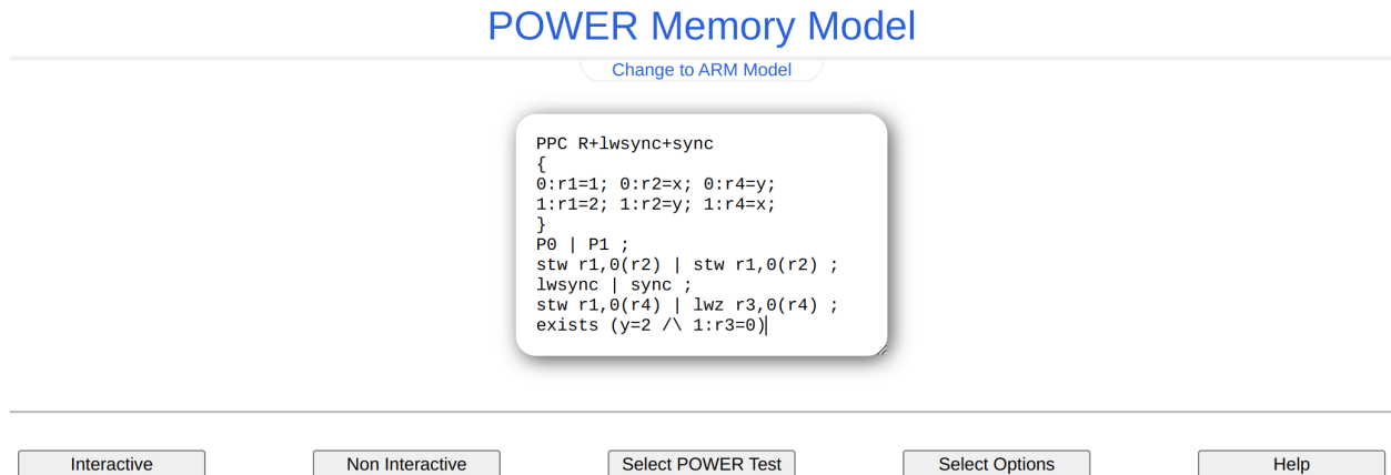
Figure 15.18: PPCMEM Initial R State
