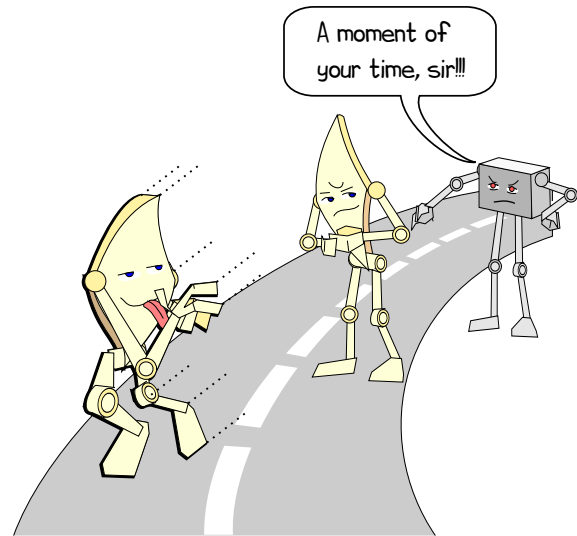
Figure 3.11: CPU, Interrupted
