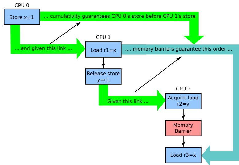
Figure 15.14: Cumulativity
