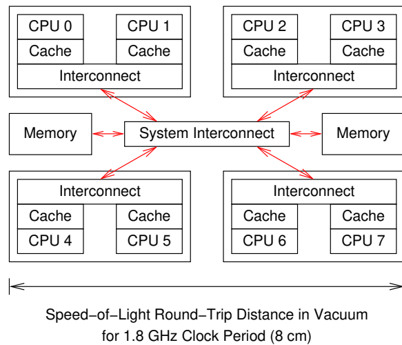
Figure 3.13: System Hardware Architecture
