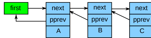
Figure 9.19: Linux Linear Linked List ( hlist )
