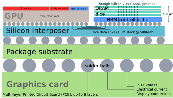
Figure 3.17: Example 3D Integration
