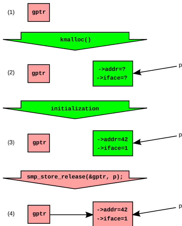
Figure 9.7: Insertion With Concurrent Readers
