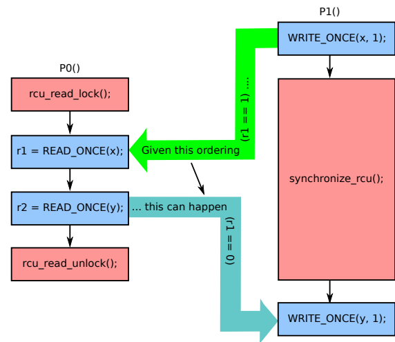
Figure 9.14: RCU Reader Within Grace Period
