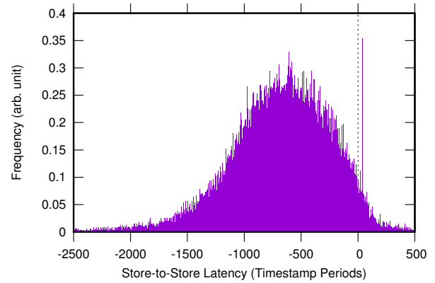
Figure E.10: Store-to-Store is Counter-Temporal on x86
