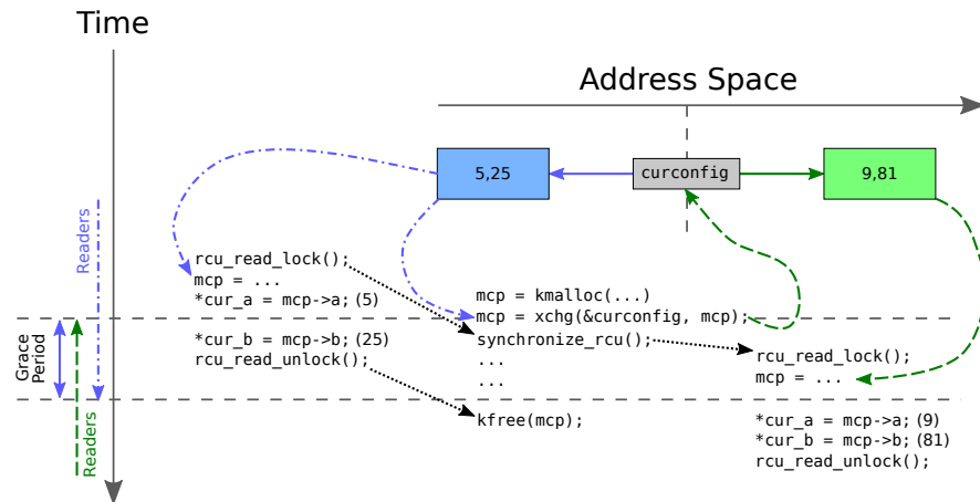
Figure 9.30: RCU Spatial/Temporal Synchronization
