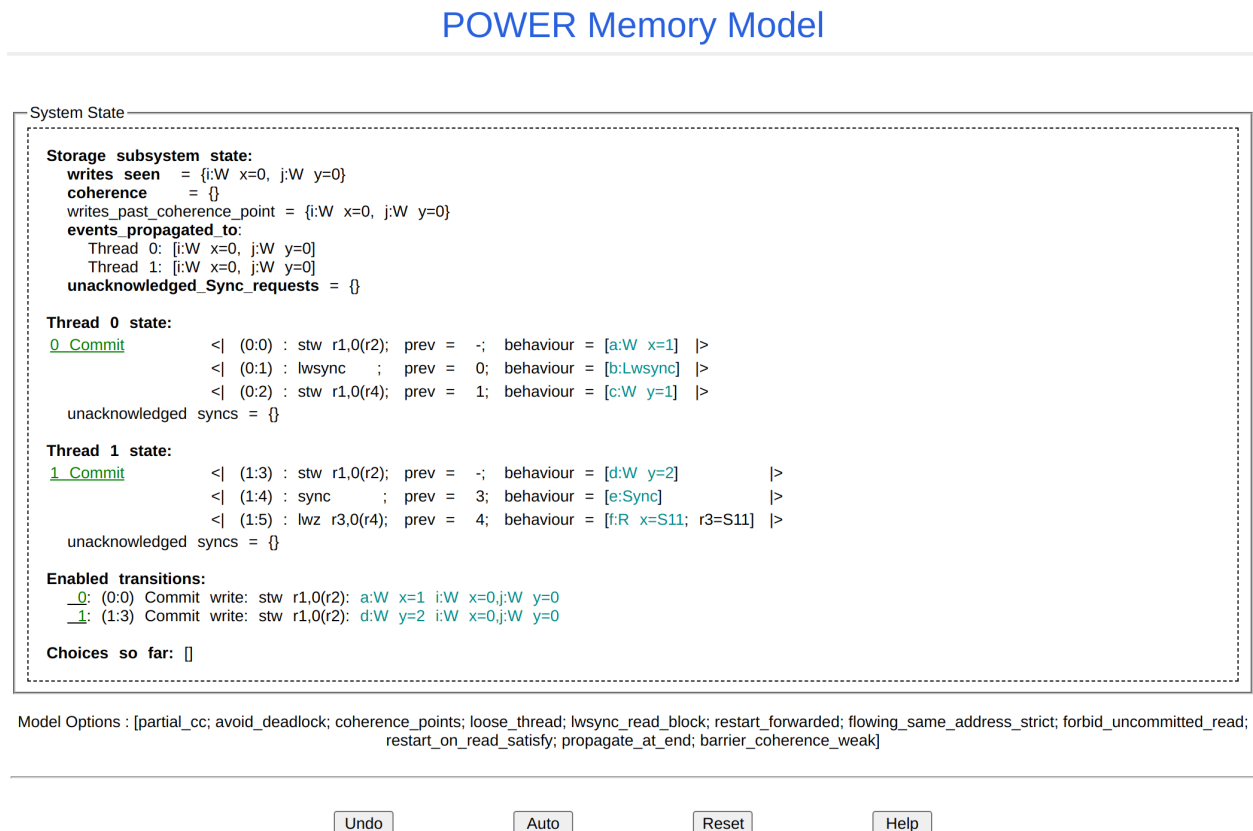
Figure 15.19: PPCMEM First R Step
