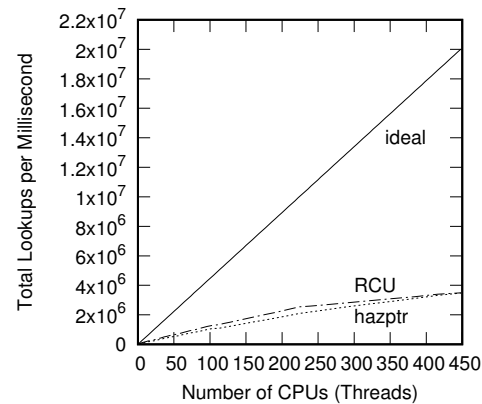
Figure 10.6: Read-Only RCU-Protected Hash-Table Performance For Schrödinger's Zoo, Linear Scale
