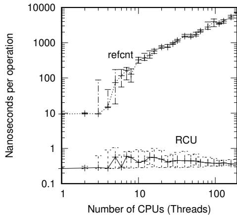
Figure 9.31: Performance of RCU vs. Reference Counting
