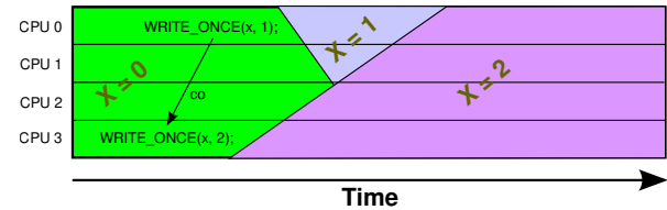
Figure 15.16: Store-to-Store is Counter-Temporal
