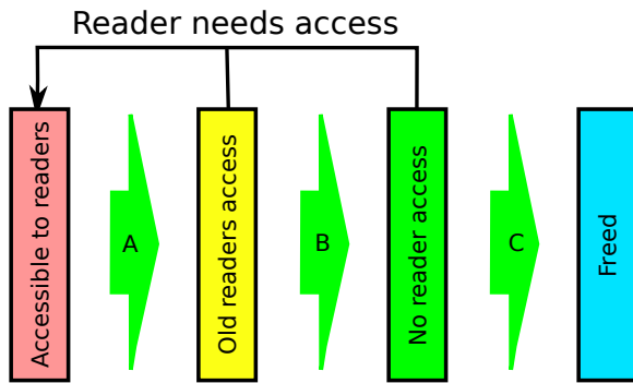
Figure 13.2: Polled RCU Cache
