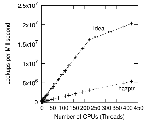
Figure 9.4: Pre-BSD Routing Table Protected by Hazard Pointers
