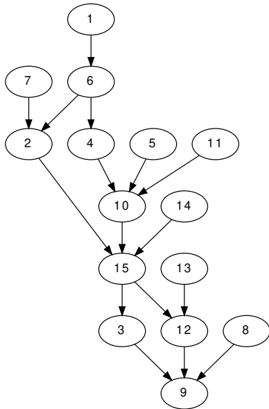
Figure 15.11: Possible Global Orders With More Simultaneous Values
