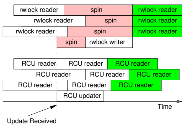
Figure 9.29: Response Time of RCU vs. Reader-Writer Locking
