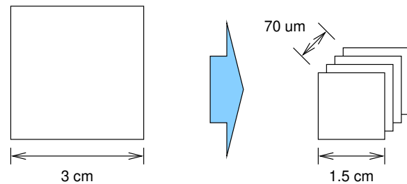
Figure 3.16: Latency Benefit of 3D Integration
