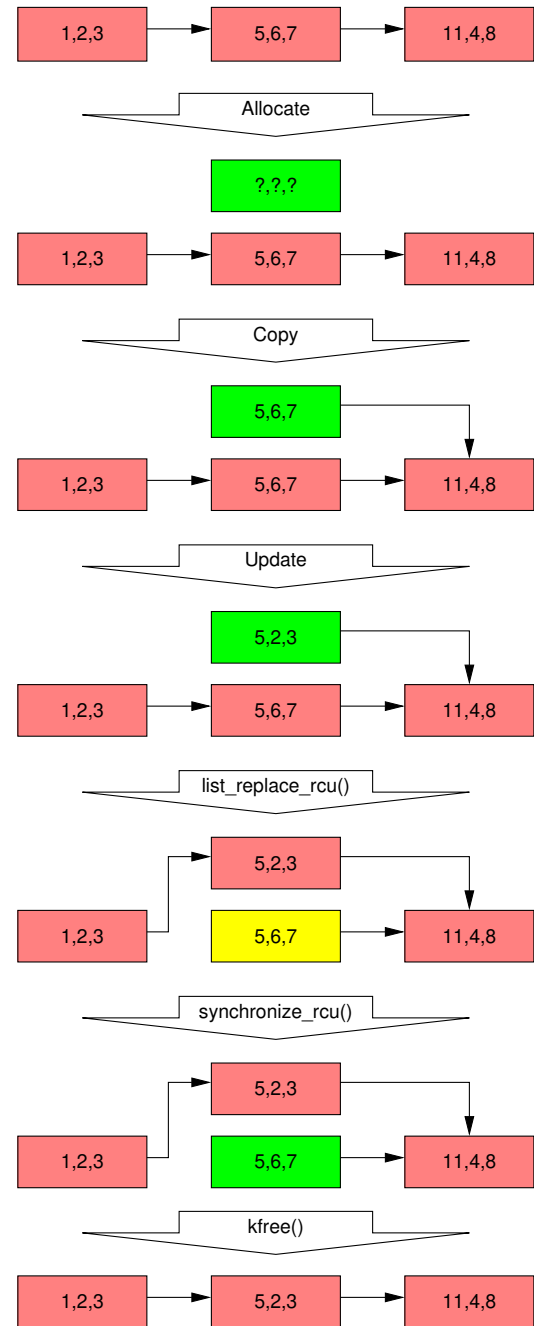
Figure 9.20: RCU Replacement in Linked List
